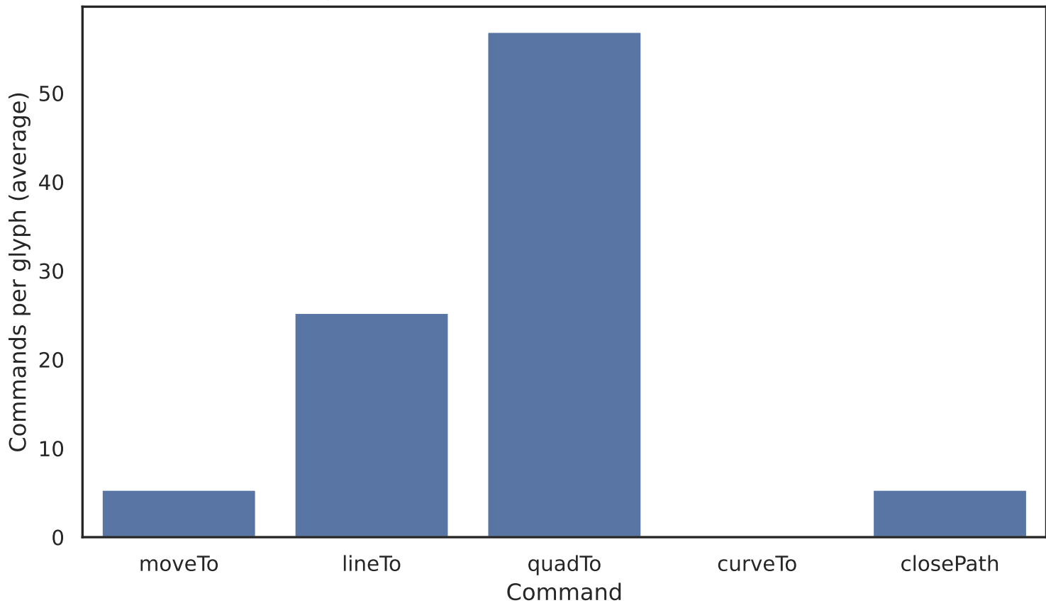
Average outline command breakdown in Google Fonts
