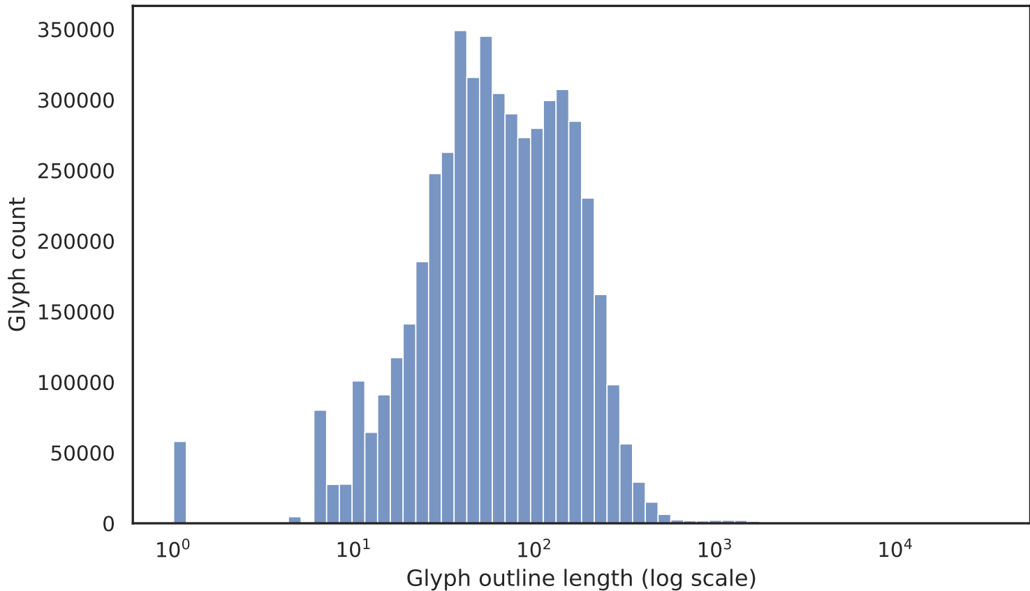
Glyph outline lengths in Google Fonts
