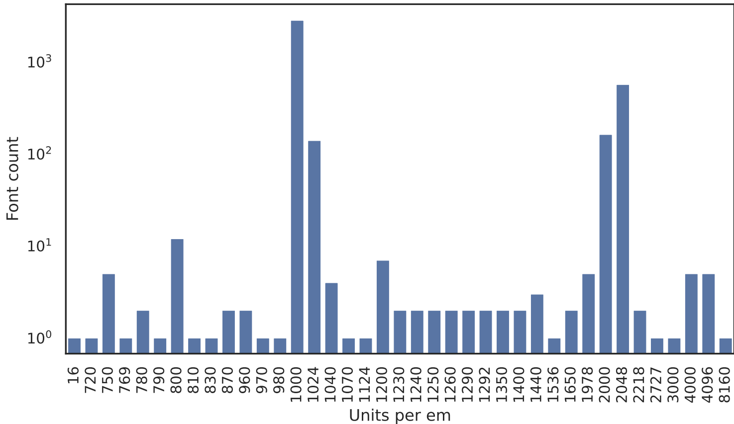
UPEM distribution in Google Fonts
